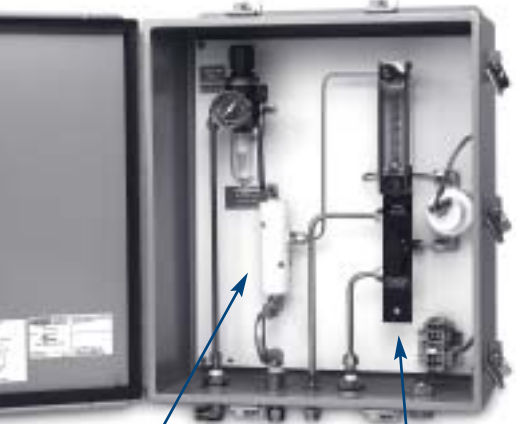
STREAMLINED OXYGEN SAMPLER WITH INTEGRATED TRANSMITTER FOR DRY POWDER/OEM APPLICATIONS
